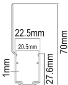
Flex Aluminum profile with shield
