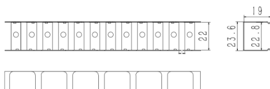
Stainless steel flexible chain
