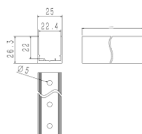
Aluminum profile
