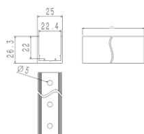
Mounting clip
