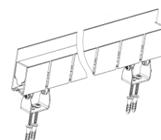
Flex Aluminum profile with shield & bracket
