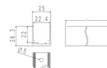
Aluminum flexible profile
