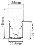
Aluminum flexible profile
